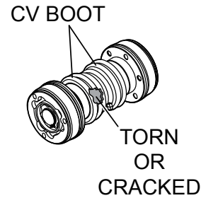
Figure 16. CV Boot Inspection
