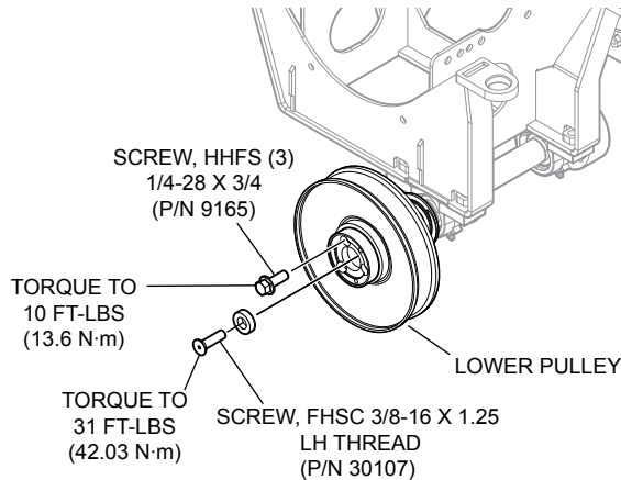
Figure 18. Lower Pulley Mounting Screw Torquing
