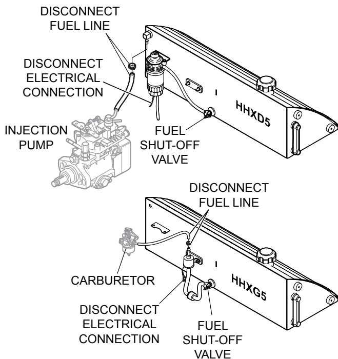
Figure 7. Disconnect Fuel Lines and Electrical Connections
