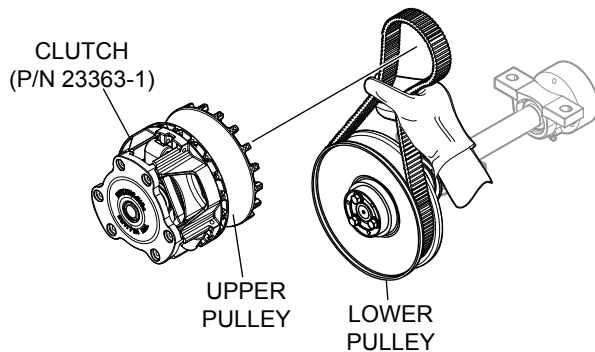
Figure 20. Upper Pulley Belt Installation
